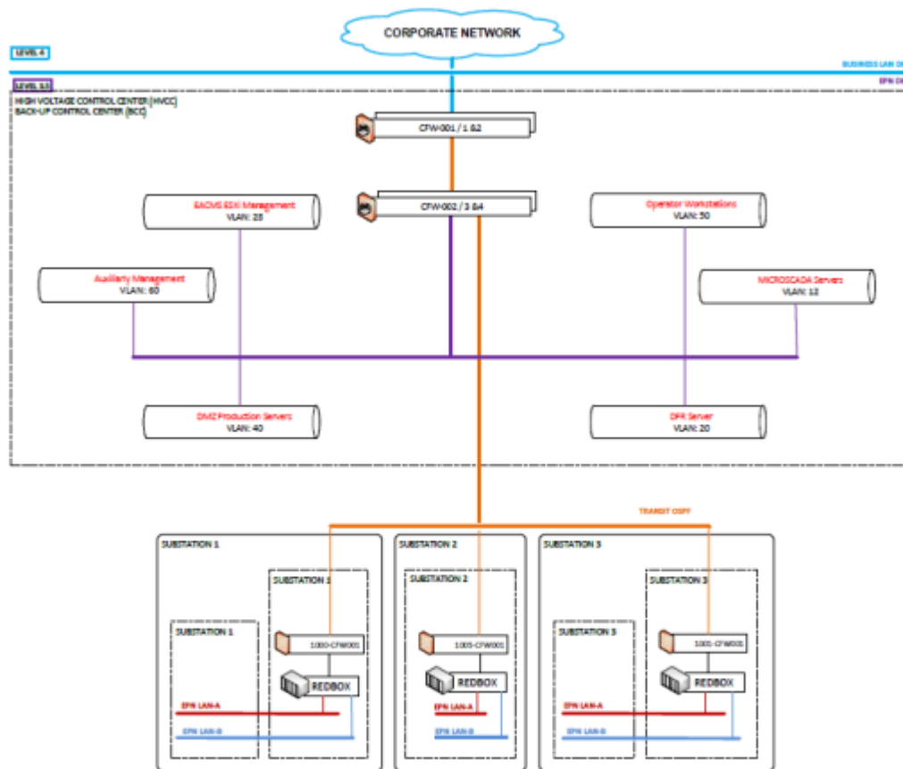
Figure 2: Network Architecture
