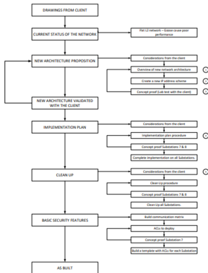
Figure 3: Segregation process
